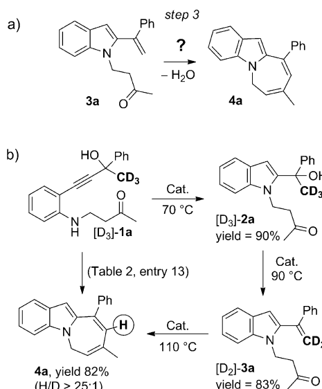
Scheme 3. a) Step 3 of the [Au] -catalyzed cyclization cascade. b) Control experiments carried out with [D_3] - 1a . Cat. = [Au(I)PrCl]/AgOTf (5 mol %).
