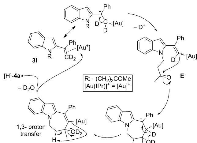
Scheme 4. Hypothetical C=C/[Au]^+ insertion leading to the formation of vinyl-gold(I) intermediate E .
